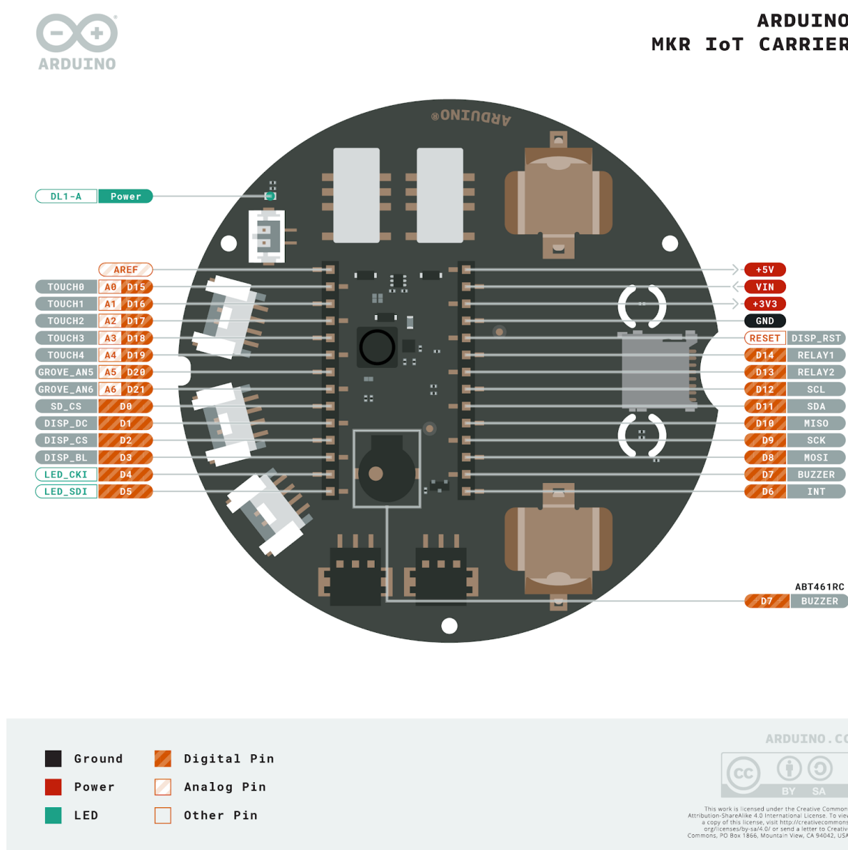
Pinout
